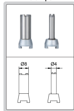
clamps
